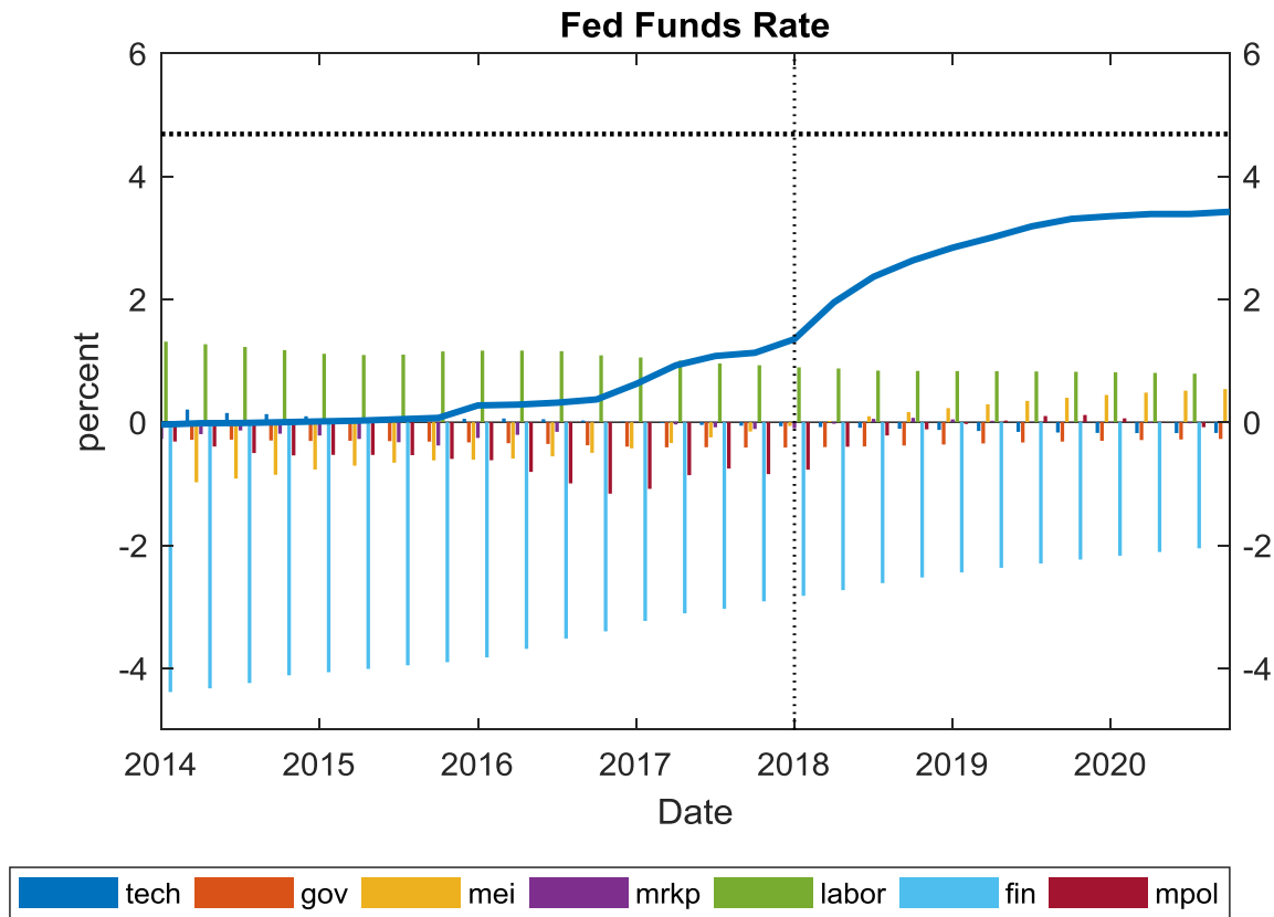
Figure 2c Shock Decompositions
