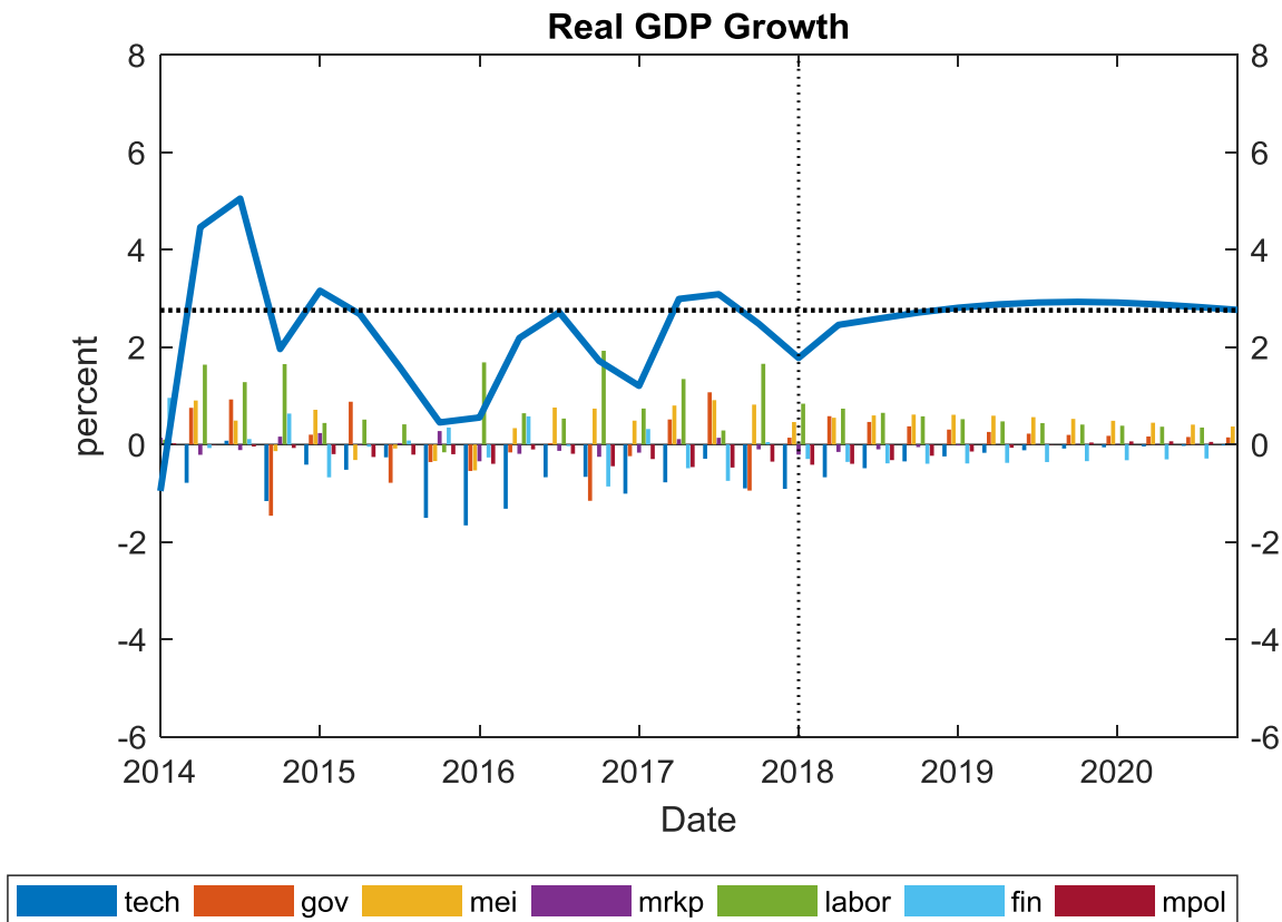
Figure 2a Shock Decompositions
