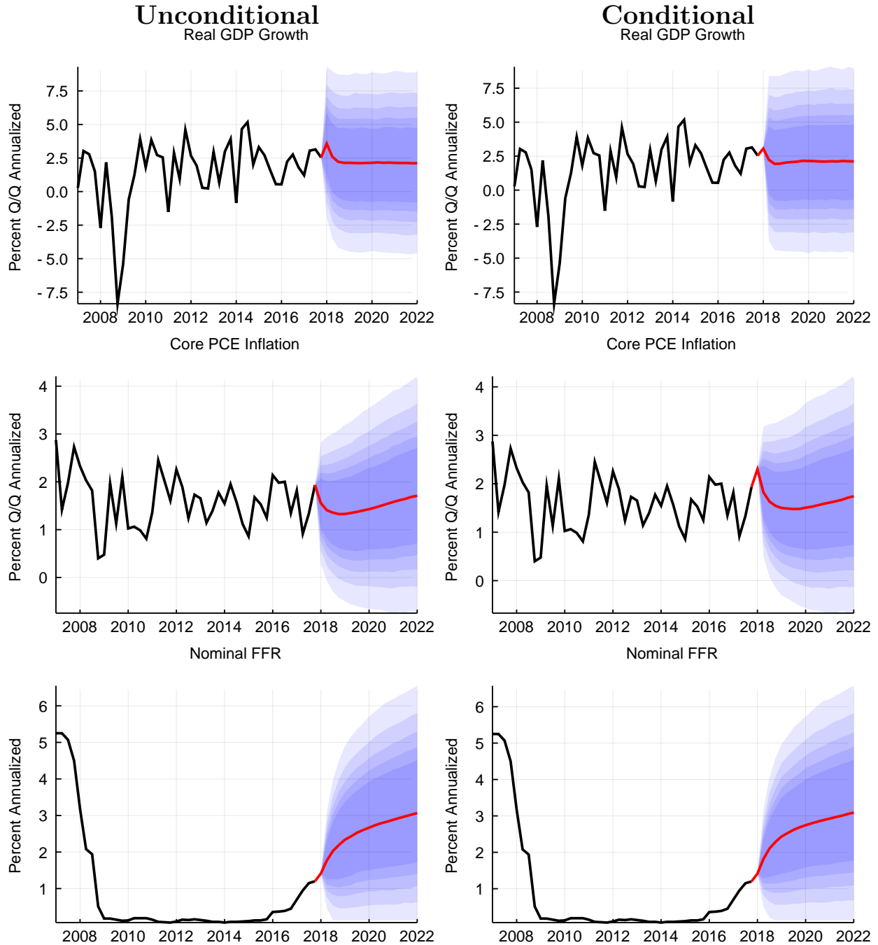
Figure 2: Forecasts
