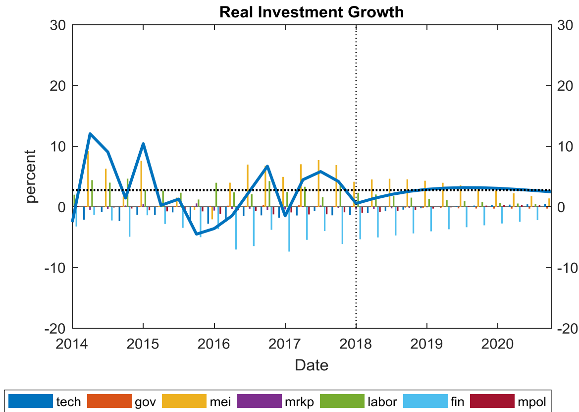
Figure 2e Shock Decompositions
