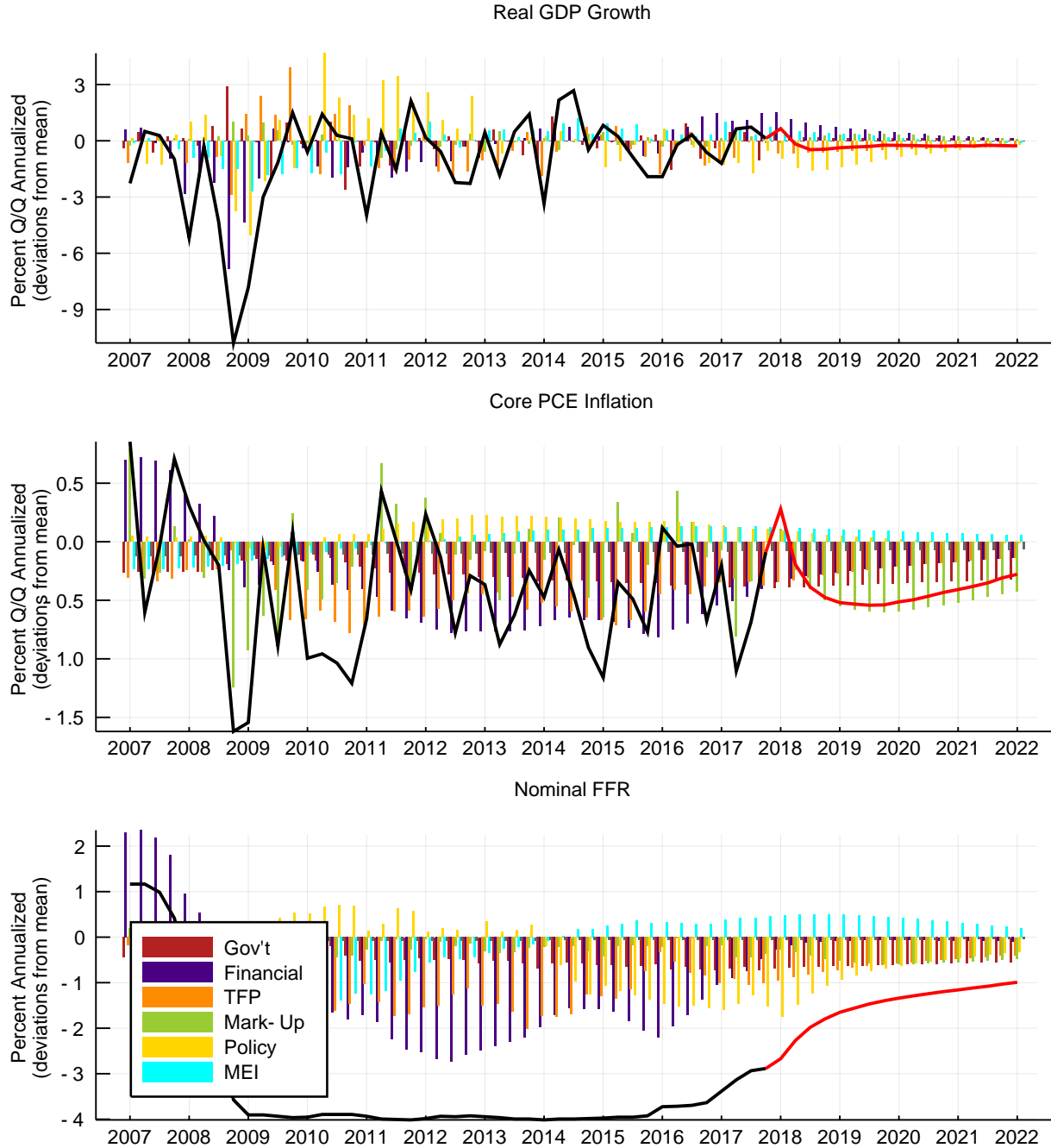
Figure 4: Shock Decomposition
